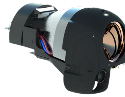
EFP WARHEAD
